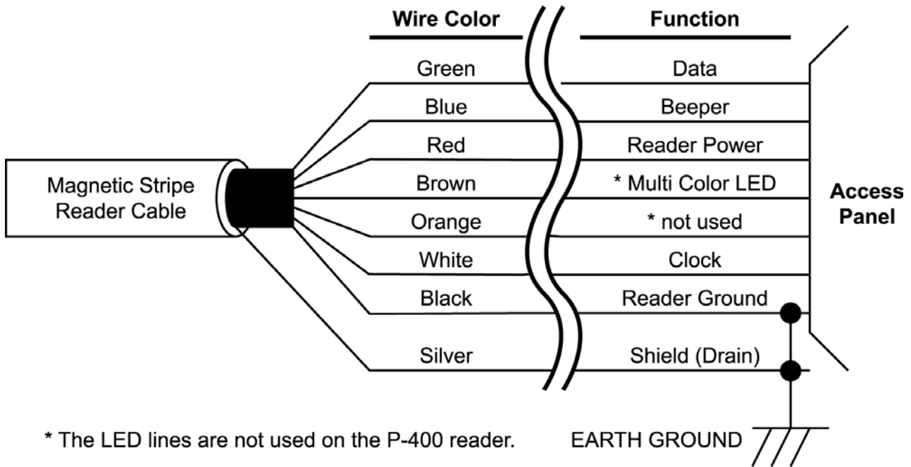
Figure 7: Magnetic Stripe Wiring Connections
