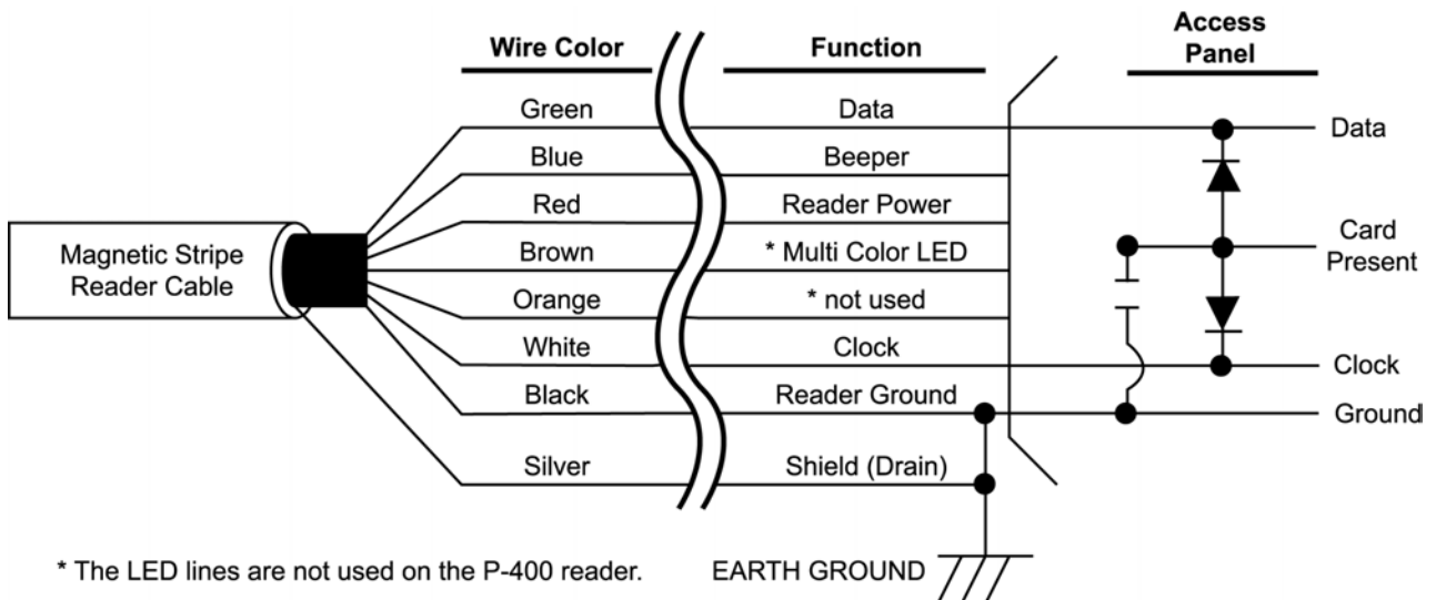
Figure 8: Magnetic Stripe Wiring Connections With Card Present Signal
