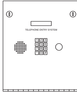
1803 Flush 12" W x 13.5" H x 2.5" D 30.4cm W x 34.3cm H x 6.35cm D
